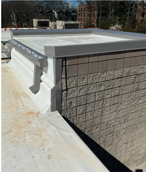
Installing new downspouts and coping
